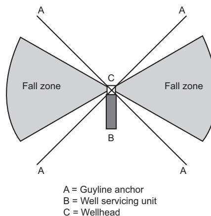
Figure 1—Guyline Anchor Locations Outside the Fall Zones
